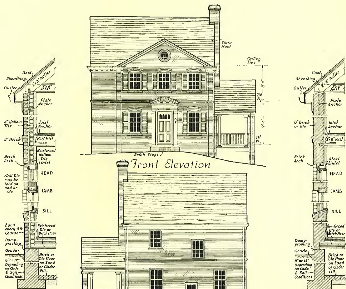
Wall Section
